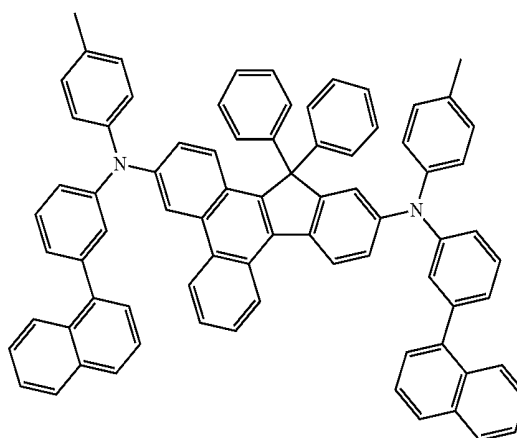
Compound 24
