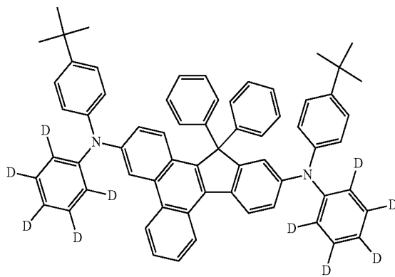
Compound 12
