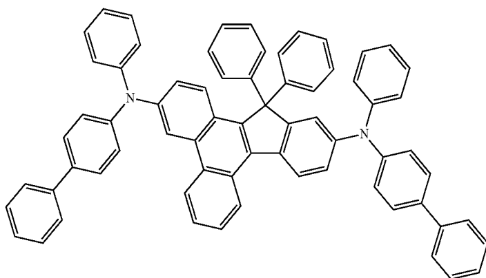
Compound 9
