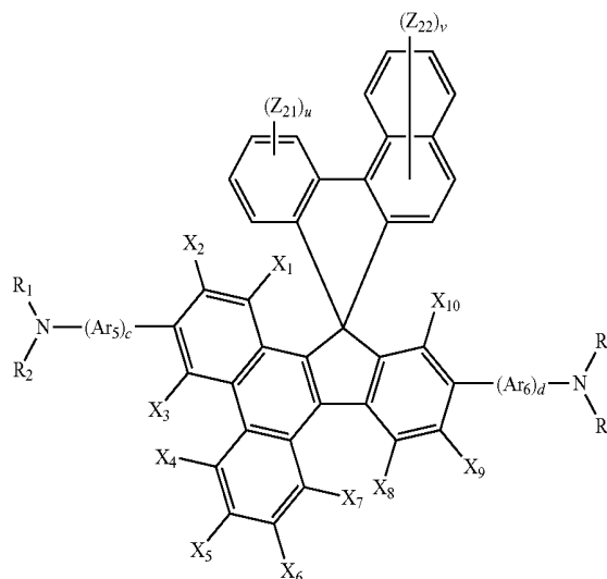
Formula 1D
