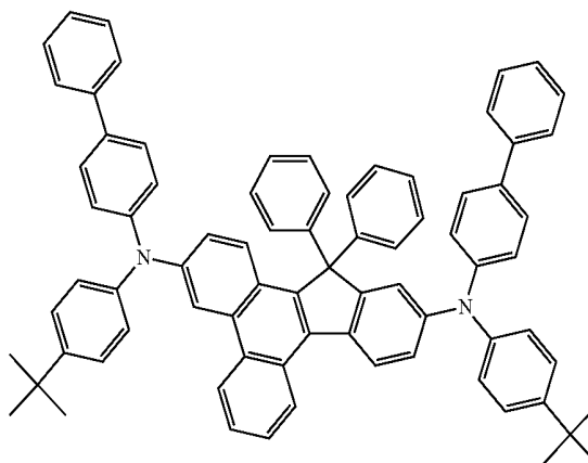
Compound 12
