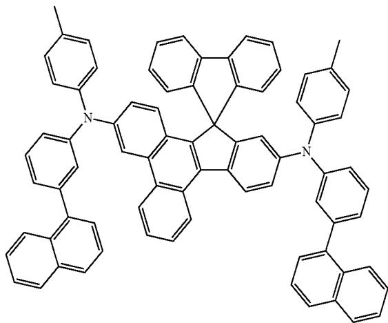
&lt;Compound 26A&gt;
