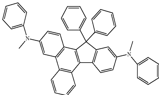
Compound 74
