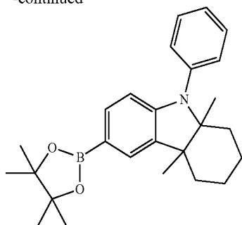
Intermediate 15-e
