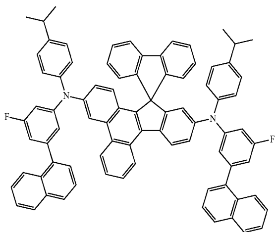
&lt;Compound 23A&gt;
