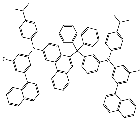
Compound 23
