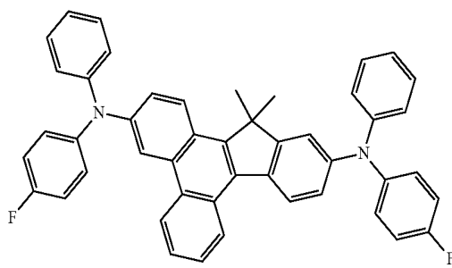
Compound 34
