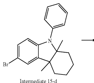
Reaction Scheme 19
