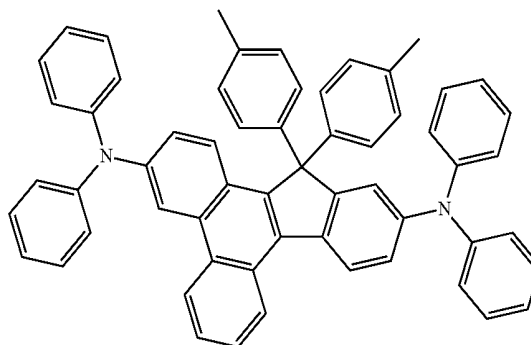
Compound 77
