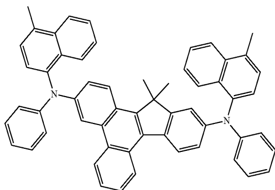
Compound 52
