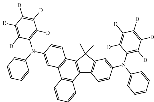
Compound 44
