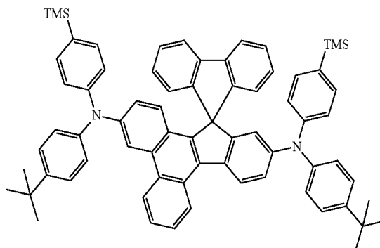
&lt;Compound 2A&gt;
