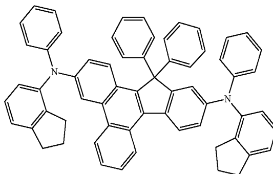
Compound 62
