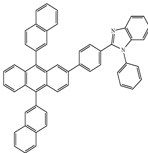
Compound 202
