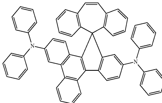
Compound 75
