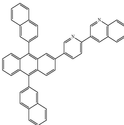
Compound 202
