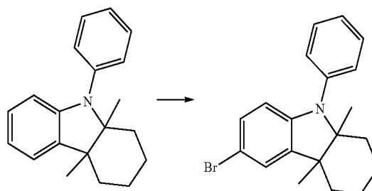
Reaction Scheme 18
