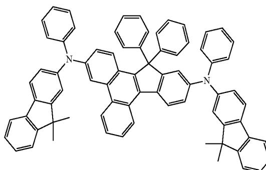
Compound 26
