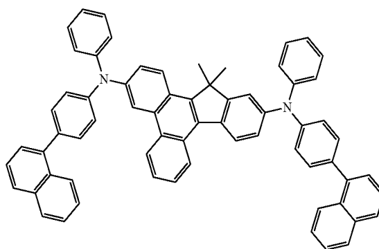
Compound 41
