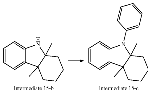
Reaction Scheme 17
