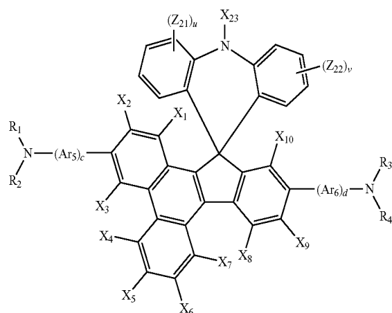
Formula 1C
