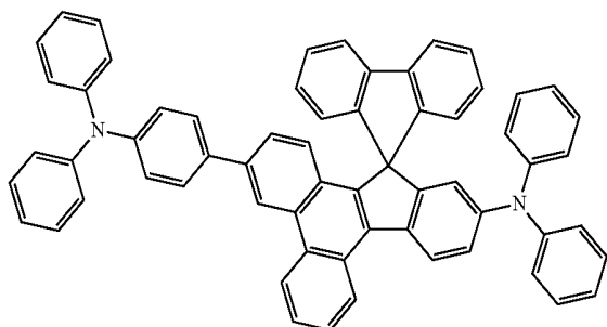
&lt;Compound 29A&gt;
