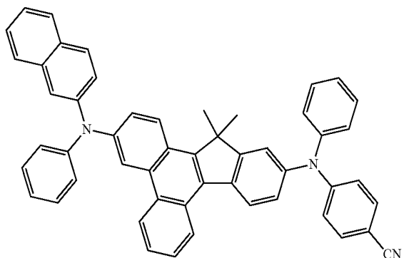
Compound 61
