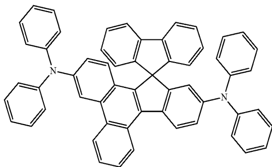
Compound 74
