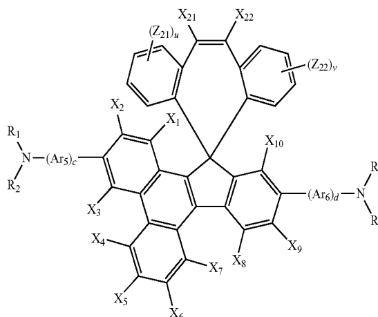
Formula 1B
