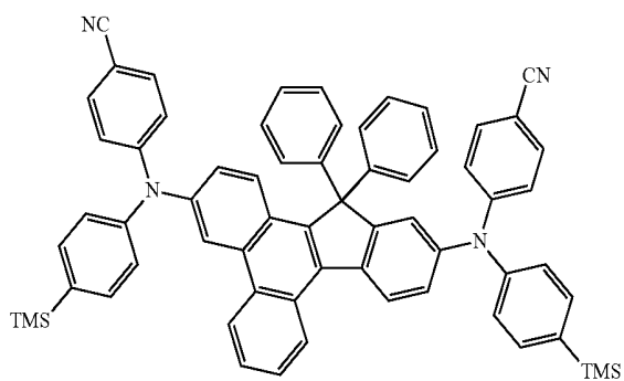
Compound 19
