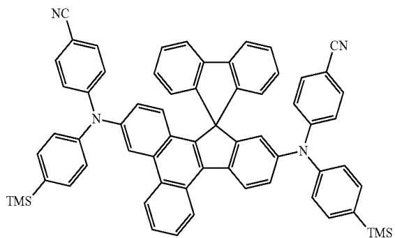
&lt;Compound 19A&gt;
