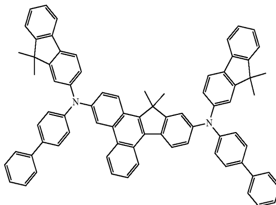
Compound 64
