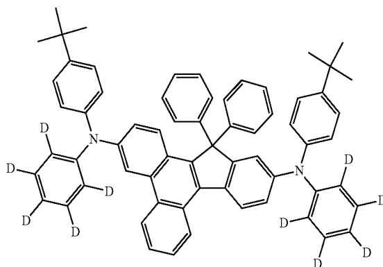
Compound 12
