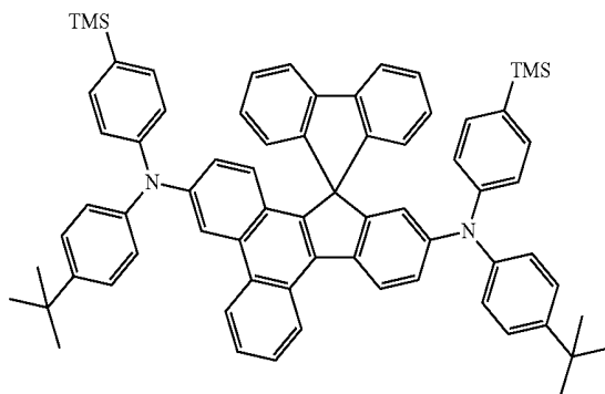
&lt;Compound 2A&gt;
