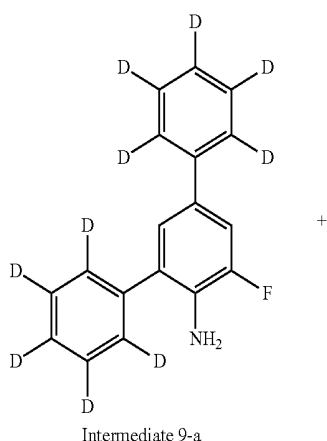
Reaction Scheme 10
