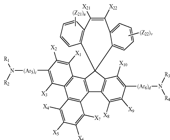
Formula 1B
