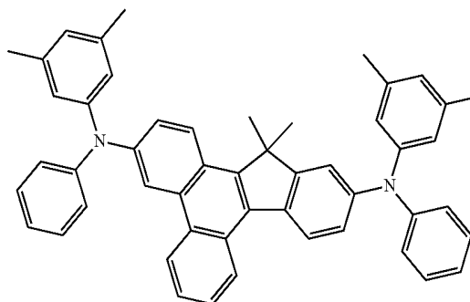
Compound 34
