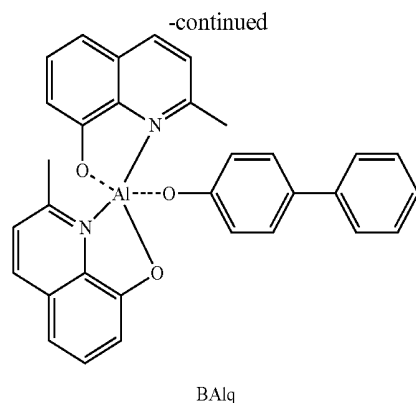
Compound 201
