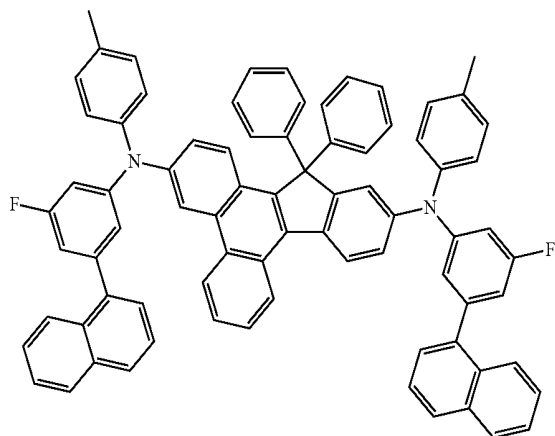
Compound 29
