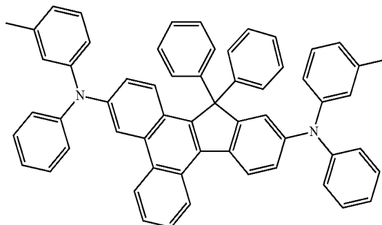
Compound 6
