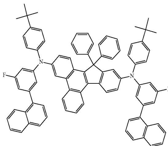
Compound 22
