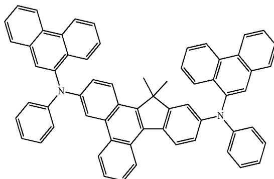
Compound 51
