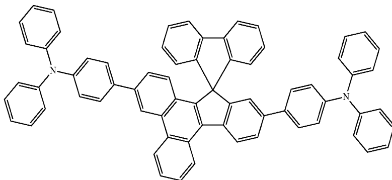
&lt;Compound 29A&gt;
