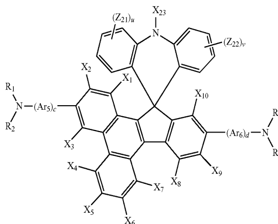
Formula 1C
