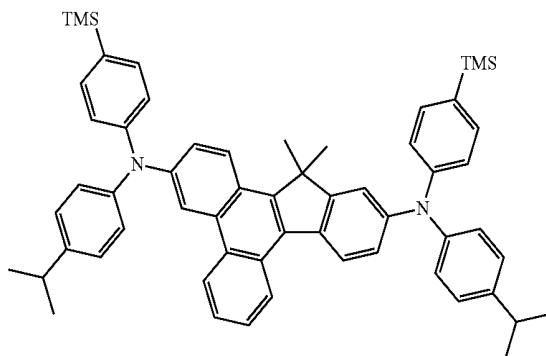
Compound 49
