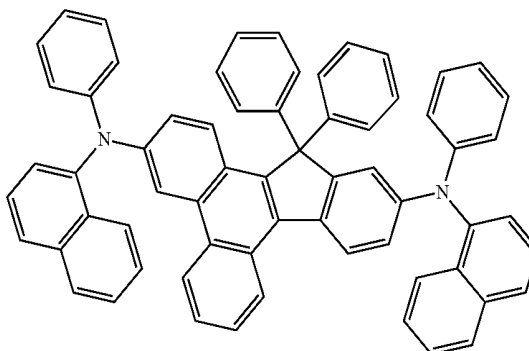
Compound 4
