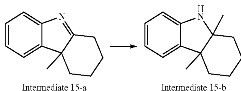
Reaction Scheme 16
