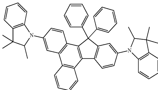
Compound 64
