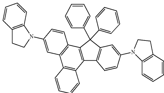
-continued Compound 63
