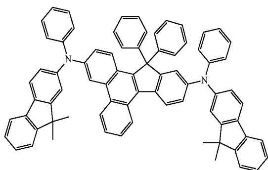
Compound 26
