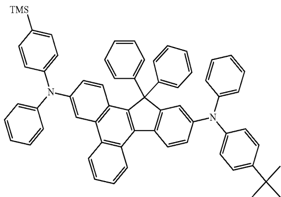
Compound 57
