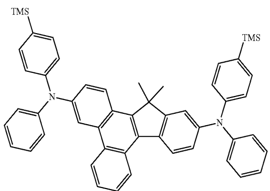
Compound 39
