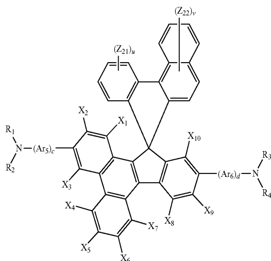
Formula 1D
