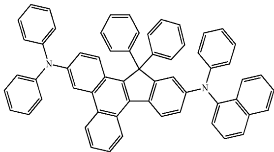
Compound 57
