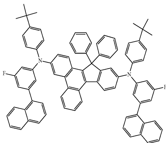
Compound 22
