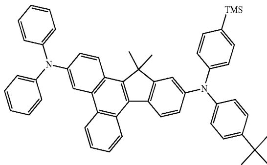
Compound 62
