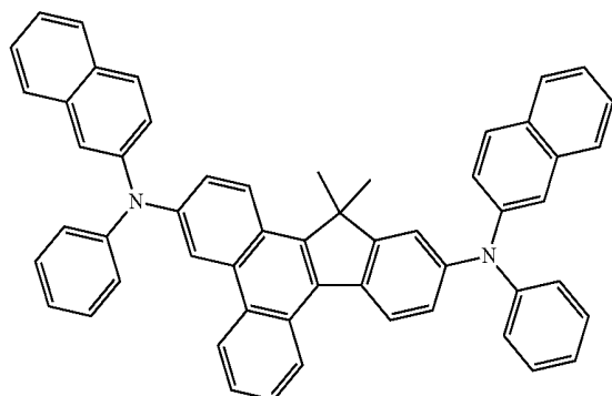
Compound 50
