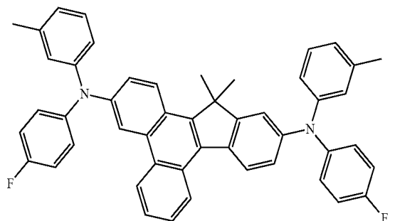
Compound 33
