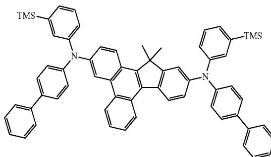
Compound 30
