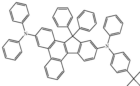
Compound 58
