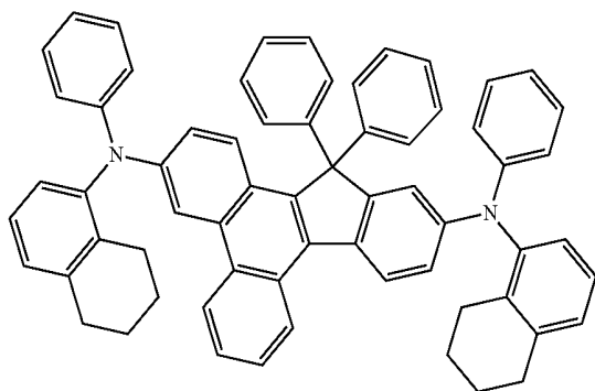
Compound 61
