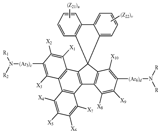
Formula 1A
