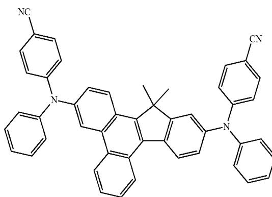
Compound 40
