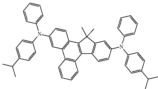
Compound 42
