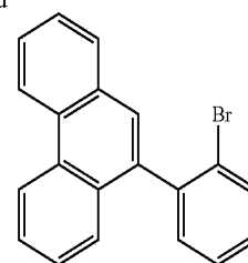
[Intermediate 2A-a]
