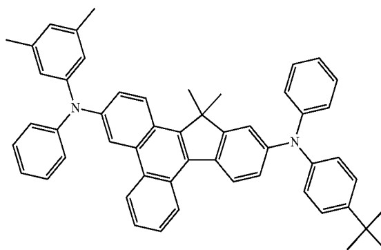
Compound 58
