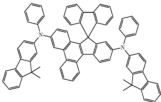
&lt;Compound 26A&gt;
