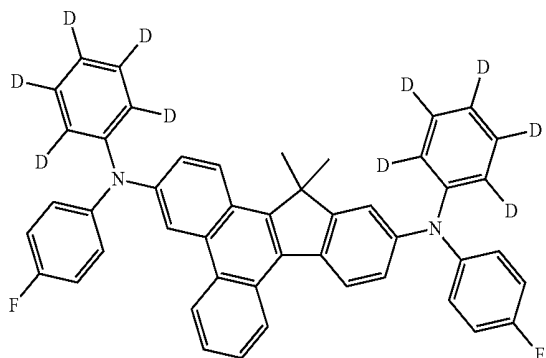
Compound 45
