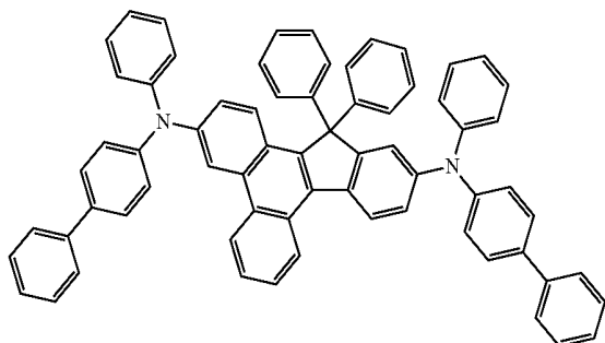
Compound 3
