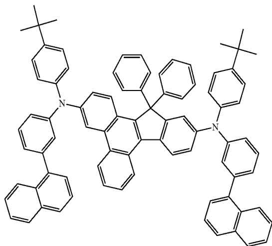
Compound 16
