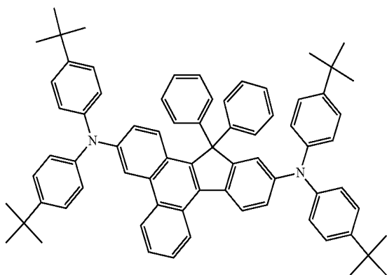
Compound 11
