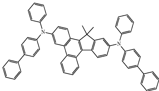
-continued Compound 29
