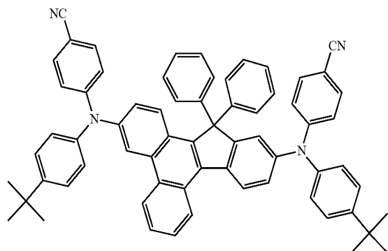
Compound 21
