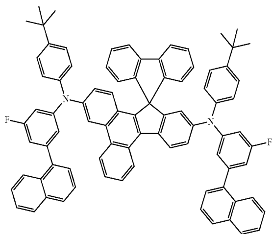
&lt;Compound 22A&gt;
