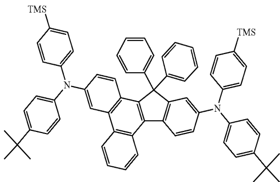
Compound 11
