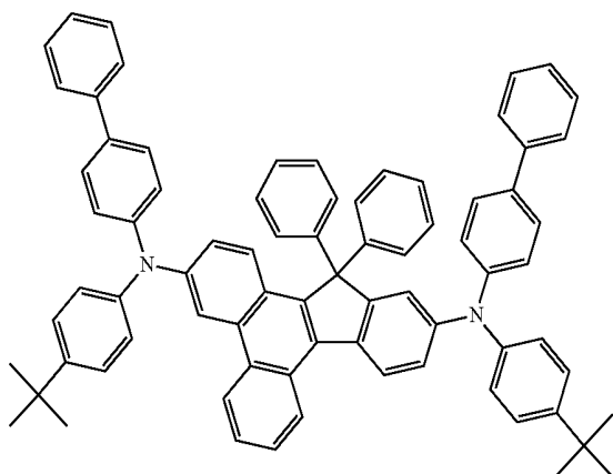
Compound 12
