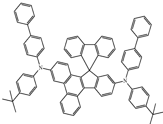
&lt;Compound 3A&gt;
