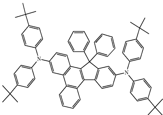
Compound 11
