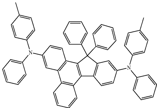
Compound 7
