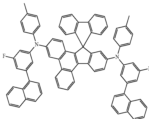
&lt;Compound 28A&gt;
