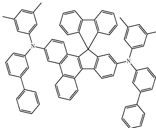
&lt;Compound 25A&gt;
