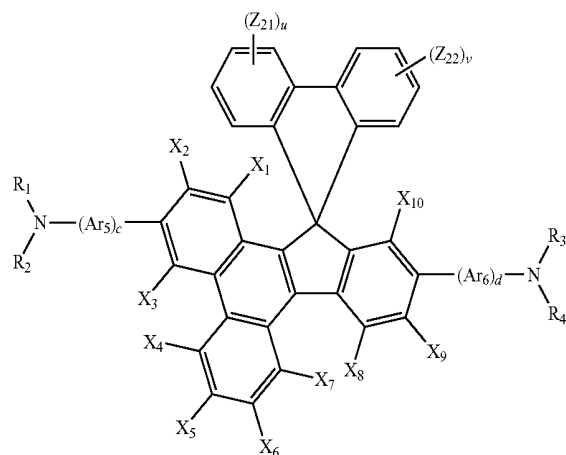
Formula 1A
