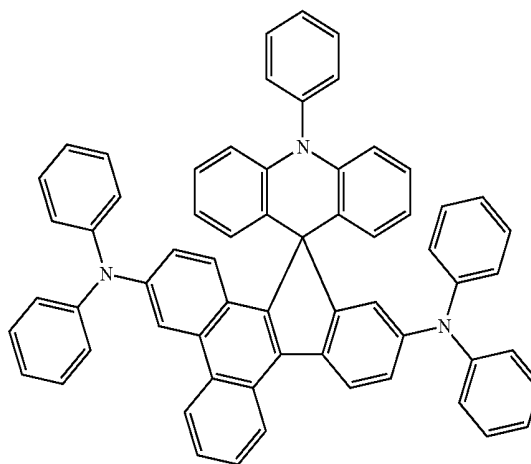
Compound 77
