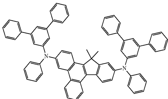
Compound 37
