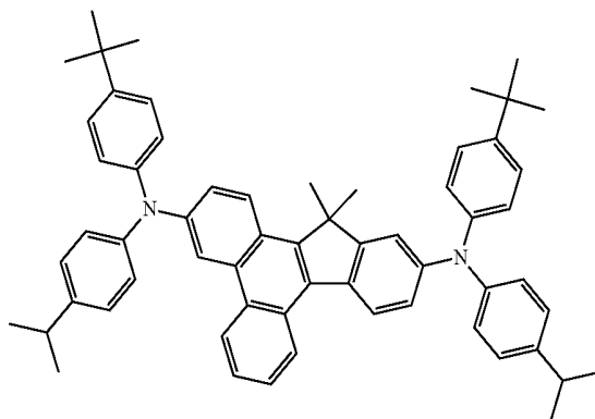
Compound 45
