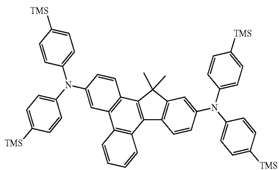
Compound 48
