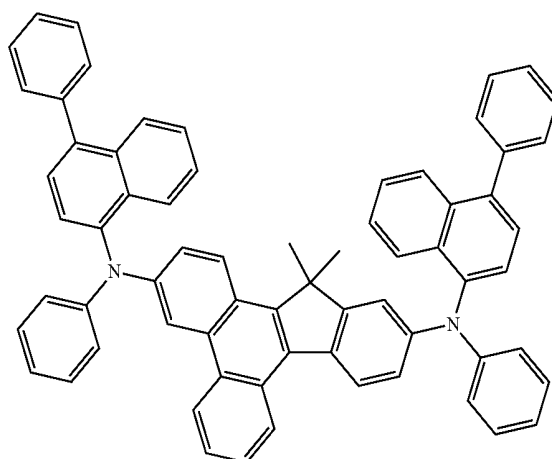
Compound 53
