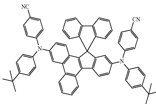
&lt;Compound 21A&gt;
